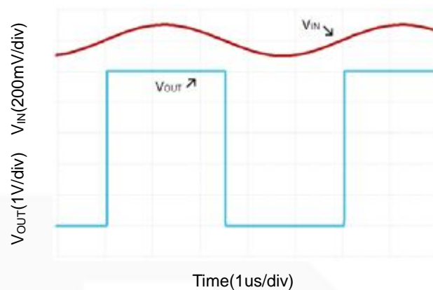
Sinusoid Response at 0.2MHz
