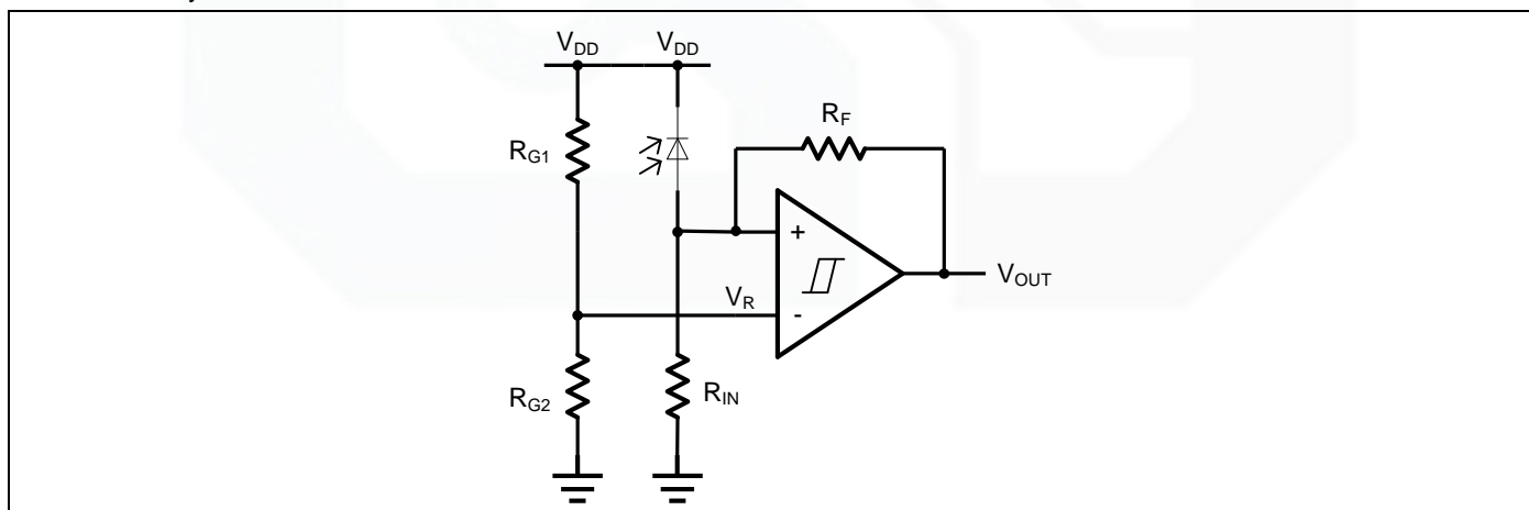
Figure 6. IR Receiver
