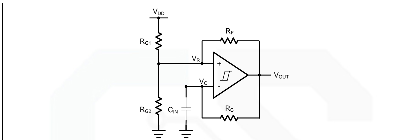
Figure 7. Oscillator
