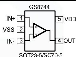
Figure 1. Pin Assignment Diagram
