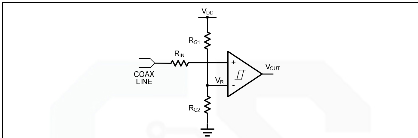
Figure 5. Line Receiver
