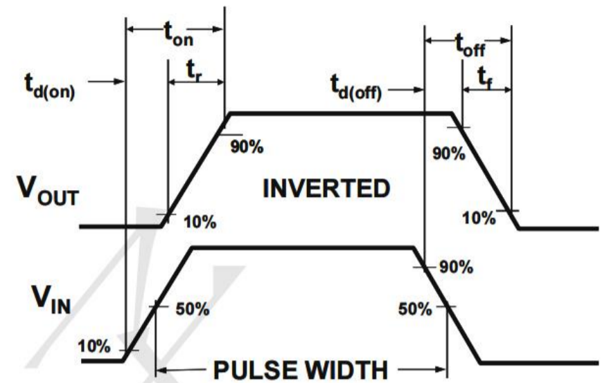
Figure 2: Switching Waveforms
