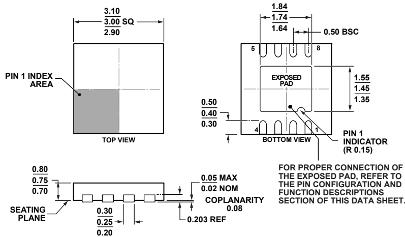
COMPLIANT TO JEDEC STANDARDS MO-229-WEED Figure 60. 8-Lead Lead Frame Chip Scale Package [LFCSP] 3 mm x 3 mm Body and 0.75 mm Package Height (CP-8-13) Dimensions shown in millimeters
